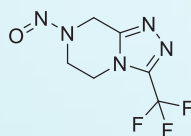
7-nitroso-3-(trifluoromethyl)-5,6,7,8-tetrahydro-[1,2,4]triazolo[4,3-a]pyrazine DCTI-C-2432
